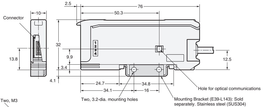
Mounting Hole Dimensions
